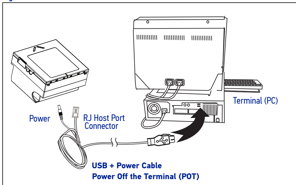
Figure 3. USB + Power Cable Power Off the Terminal
