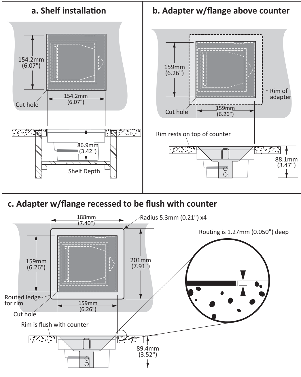
Figure 6. Countertop Cutouts
