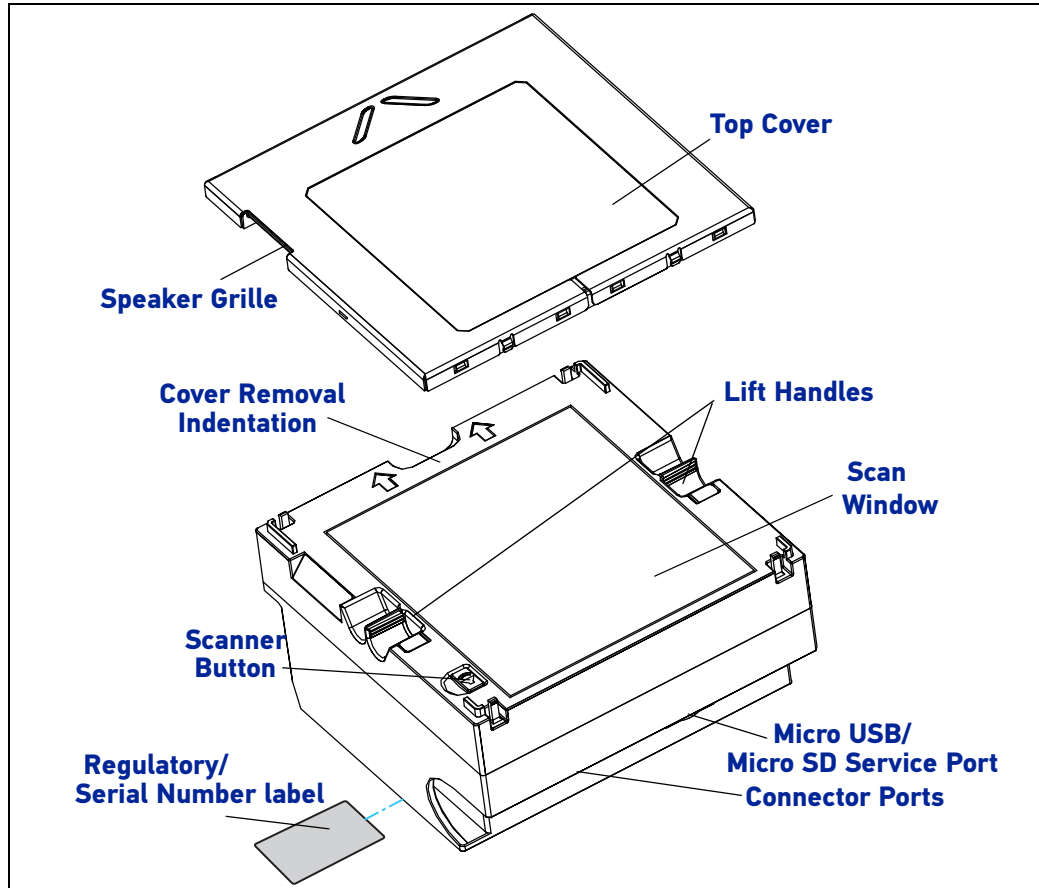
Figure 1. Scanner Features - Front View
