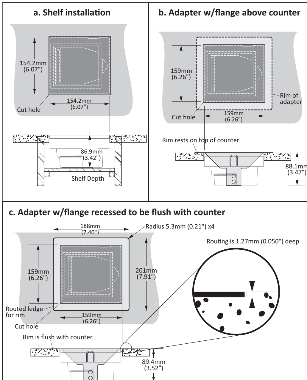
Figure 5. Countertop Cutouts
